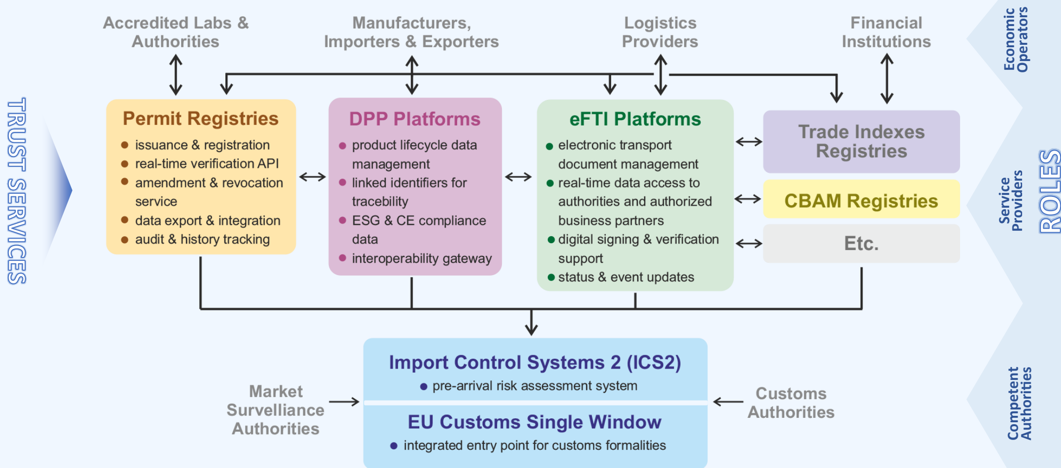
Figure 1. This diagram illustrates the key platforms, data flows, and stakeholder interactions across the EU's digital trade and customs ecosystem. It shows how manufacturers, logistics providers, and regulatory systems connect through structured data platforms—such as eFTI, the Digital Product Passport, and EU Customs systems—while integrating with trusted external sources including TRACES, REACH-IT, and EUDAMED. Trust Services supporting this interoperability include LEI/vLEI, Qualified Electronic Signature, Qualified Electronic Seal, Qualified Timestamp, etc. All data exchanges comply with the General Data Protection Regulation (GDPR) . The diagram was prepared by Riho Vedler and is presented on behalf of the DigitalTrade4.EU consortium.
